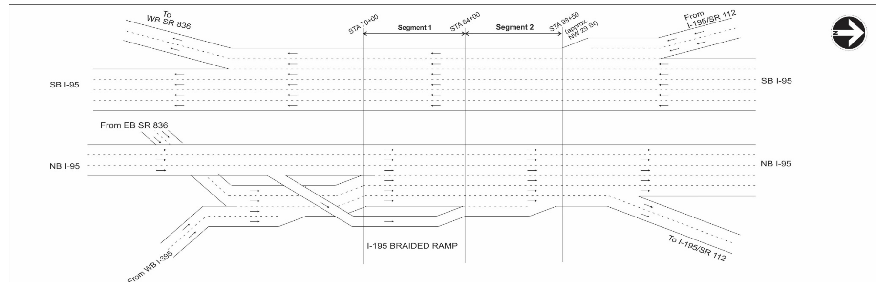
Figure 4-2: Freeway Segments Schematic – I-95
